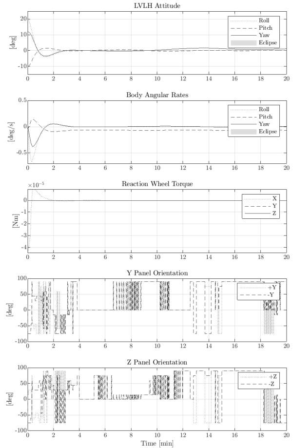
Figure 11: Performance of the aerodynamic pointing manoeuvre about the pitch & yaw axes for SOAR. Motion about the roll axis is controlled by the RWS. After the initial offset is nulled out, the aerodynamic panels are still employed to reject external disturbances in pitch and yaw.
